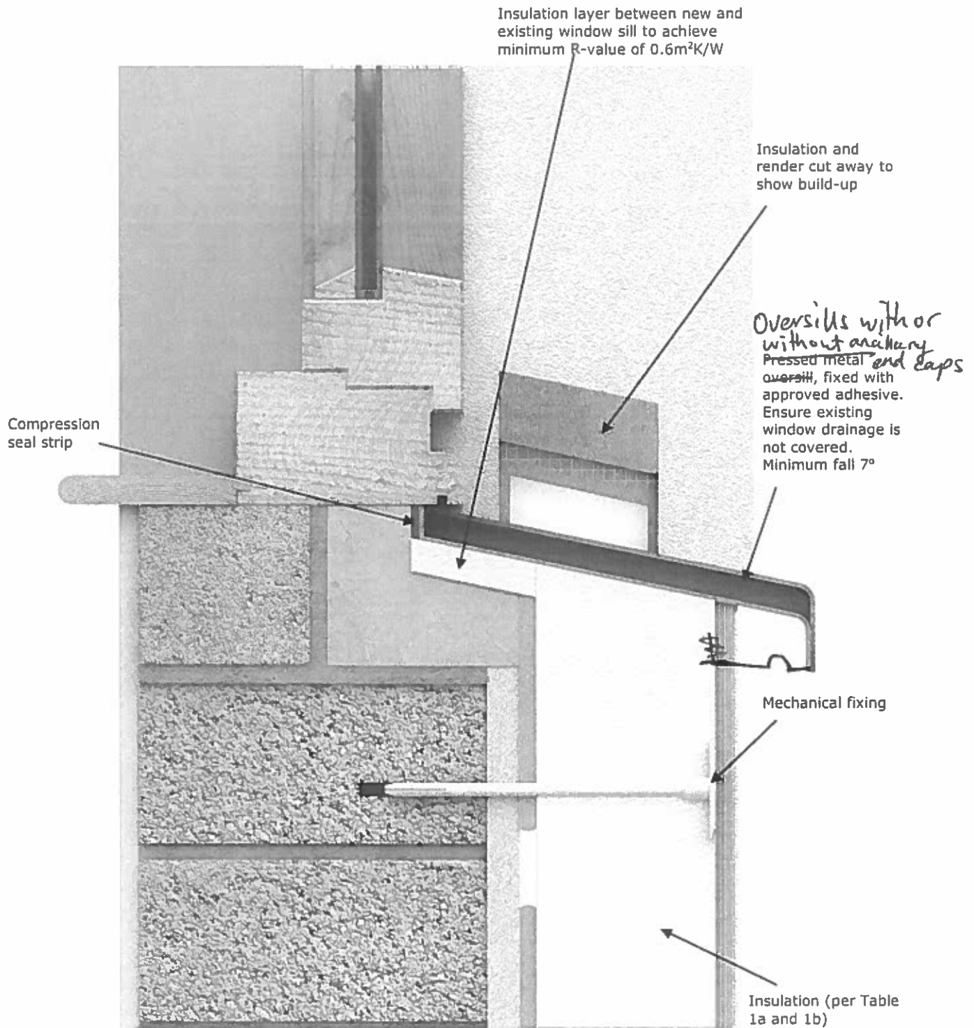
Figure 2: Window Sill Detail
