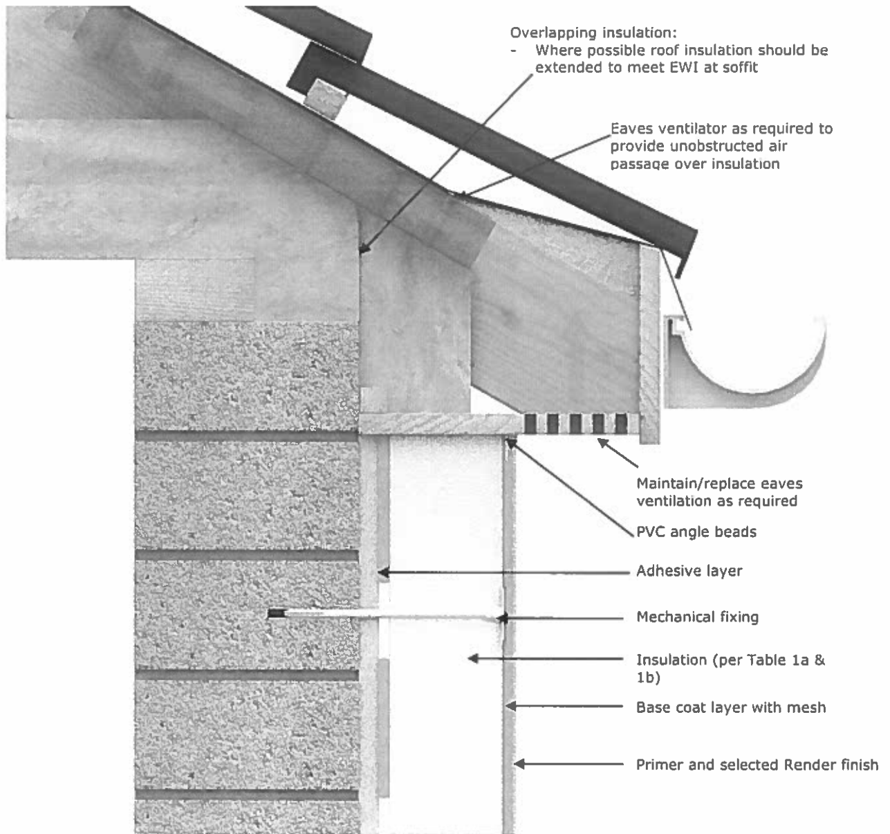
Figure 5: Eaves Detail
